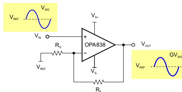
Figure 61. Noninverting Amplifier
