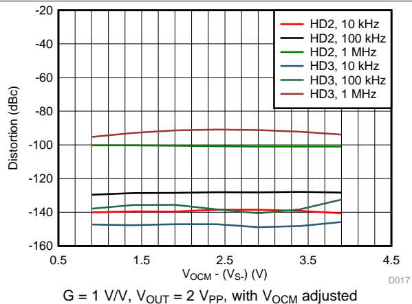
Figure 17. Harmonic Distortion vs V_{OCM}
