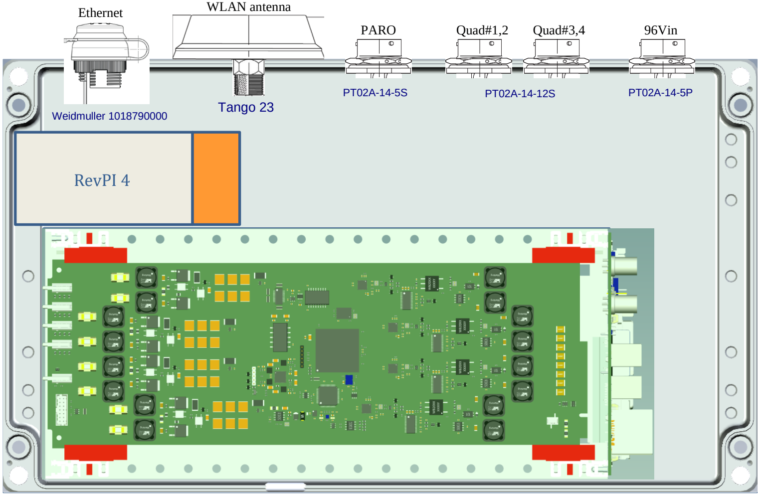
SpoolHub, Top View, scale 1:2, version #2, 2x2 quad conns. vertically aligned
