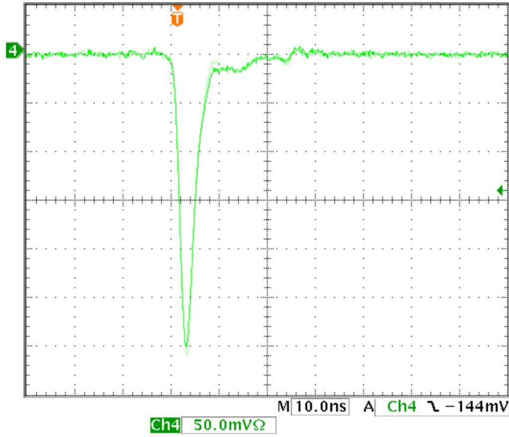
PMT pulse measured, using 403nm UV-LED OCU 400 403
