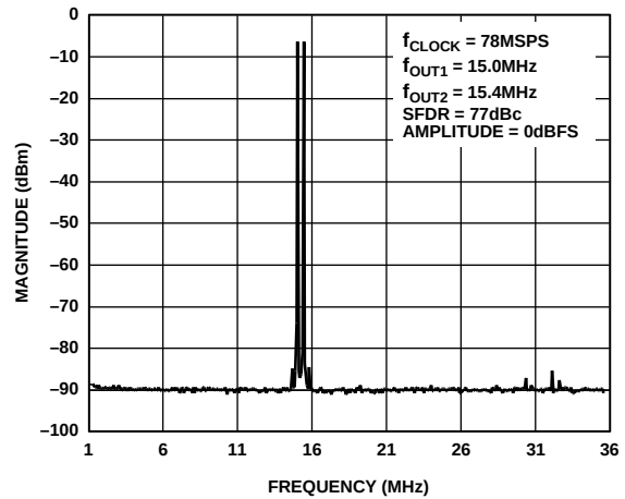
Figure 19. Dual-Tone SFDR
