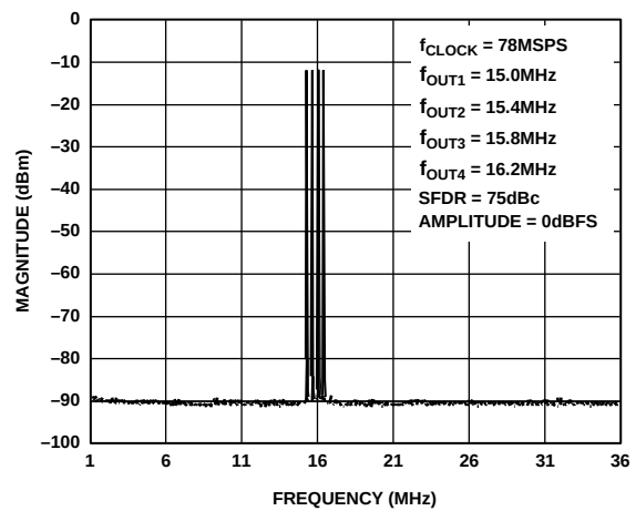
Figure 20. Four-Tone SFDR
