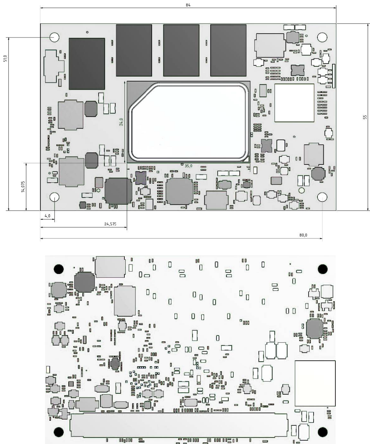
Figure 7: Module Dimensions
