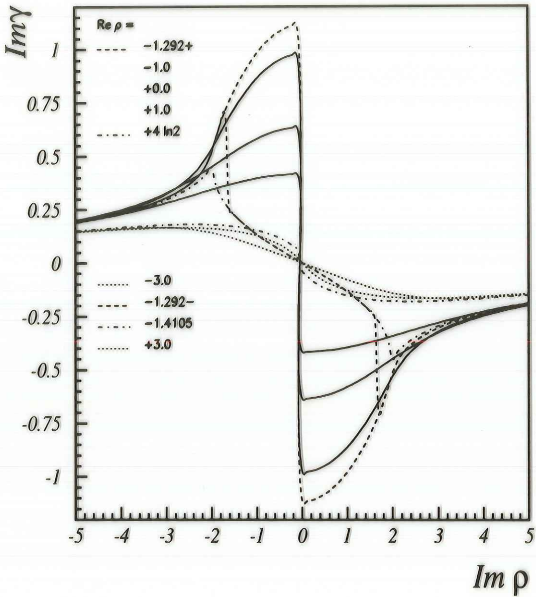
Figure 1b: Imaginary part of \gamma_L(\rho) for -3 \leq Re \rho \leq 3 and -5 \leq Im \rho \leq 5 . The notations are the same as in figure 1a.
