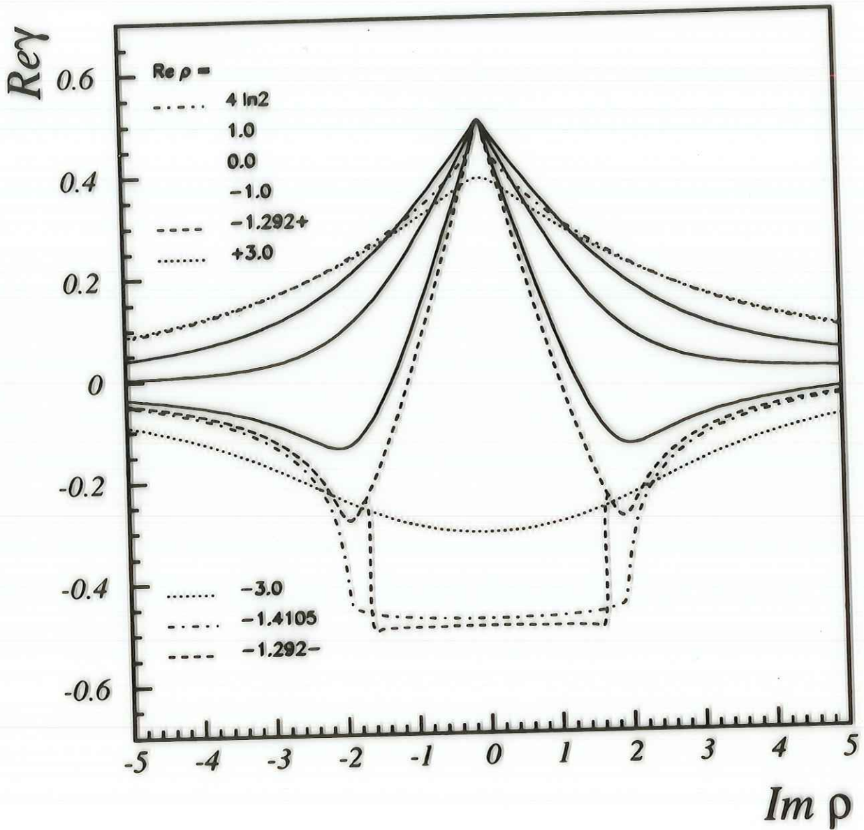
Figure 1a: Real part of the perturbative branch of \gamma_L as a function of the real and imaginary part of \rho = N/\bar{\alpha}_s . The full lines correspond to Re \rho = 1, 0, -1 and the dash-dotted lines are the contours through the singularities.
