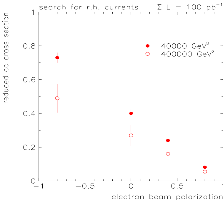
Figure 1.2.16: Search for right-handed currents in CC scattering at THERA using a measurement of the electron-proton CC cross section as a function of the electron beam polarisation, \lambda . This simulation assumes a total integrated luminosity of 100\text{pb}^{-1} distributed over four measurements at different \lambda .
