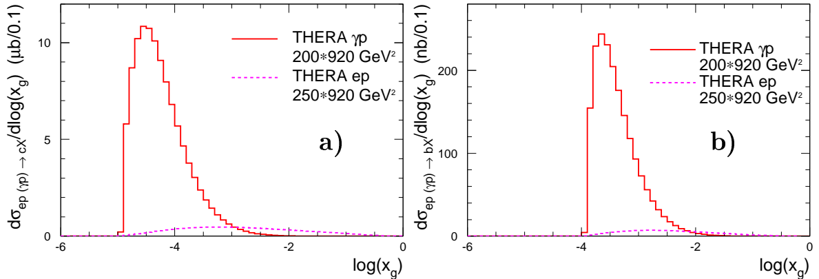
Figure 1.4.3: Dependence of the differential cross section of (a) charm and (b) beauty production on x_g in \gamma p and ep scattering at THERA.
