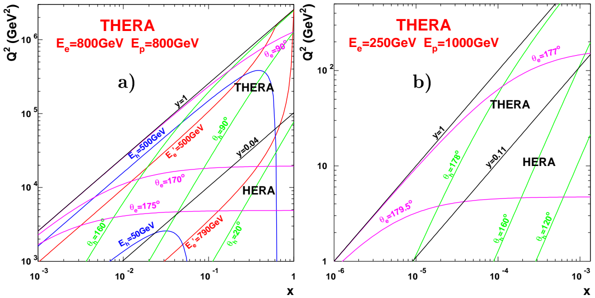
Figure 1.3.3: Kinematic range covered by THERA, (a) at high x and Q^2 for E_e = E_p = 800\text{ GeV} ( \sqrt{s} = 1.6\text{ TeV} ), and (b) at low x and Q^2 for beam energies of E_e = 250\text{ GeV} and E_p = 1\text{ TeV} ( \sqrt{s} = 1\text{ TeV} ). The lines for y = 0.04 in (a) and y = 0.11 in (b) indicate the kinematic limit of HERA. Lines of constant E'_e (red), E_h (blue), \theta_e (magenta) and \theta_h (green) are indicated. In (b), E_h and E'_e are given approximately by yE_e and (1-y)E_e , respectively. Note that for low x both the electron and the jet are scattered into the backward region, illustrating the strong boost of the electron–quark system in this kinematic region.
