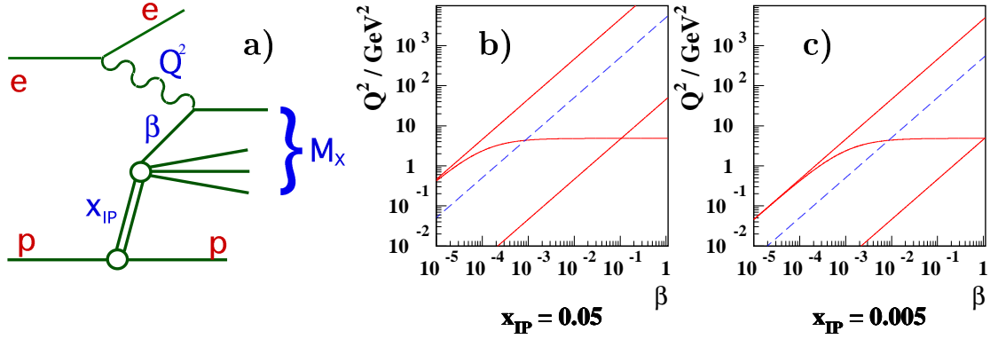
Figure 1.2.5: (a) Feynman diagram of diffractive ep scattering, with the kinematic quantities indicated in blue. (b,c) The accessible kinematic plane in \beta and Q^2 for diffractive DIS at two different values of x_{\text{IP}} . The solid red lines show the limits imposed by the cuts 0.001 < y < 1 and \theta_e < 179.5^\circ for THERA, with electrons of 250 GeV and protons of 920 GeV. The dashed blue lines show the kinematic limit at HERA.
