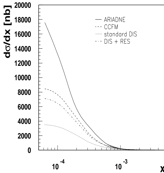
Figure 1.2.9: Forward-jet cross section as a function of x in different models for 0.5 < p_t^2/Q^2 < 2 and a minimum polar jet angle of 1^\circ . The measurements at HERA are limited to x \gtrsim 2 \times 10^{-3} .
