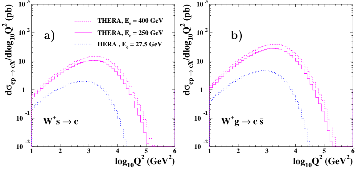
Figure 1.2.14: The differential cross sections d\sigma/d\log_{10} Q^2 for charm production in charged current DIS, (a) from the strange sea and (b) from boson–gluon fusion, calculated with the LO Monte Carlo generator HERWIG. The cross sections are shown for THERA for a proton beam energy of 920 GeV and electrons with 250 GeV (solid magenta) and 400 GeV (dashed magenta), and for HERA (dashed blue).
