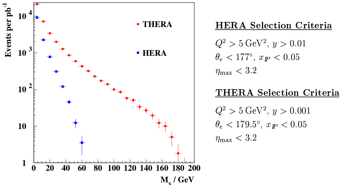
Figure 1.2.7: Event yields per unit luminosity for the process ep \rightarrow eXp after applying the quoted selection criteria at THERA (920 GeV protons, 250 GeV electrons) and HERA. The yields are shown as a function of the mass M_X and are based on an ad hoc extrapolation of a QCD fit to HERA data [42].
