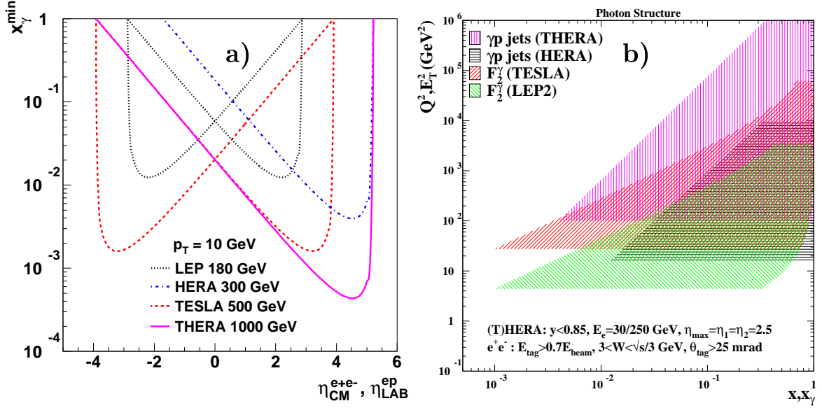
Figure 1.2.19: (a) The minimum photon momentum fraction, x_\gamma^{\min} , as a function of the rapidity in the centre-of-mass frame for e^+e^- colliders and in the laboratory frame for ep colliders. (b) Range in Q^2 ( Q^2 or p_T^2 ) versus x or x_\gamma with kinematic cuts reflecting a realistic detector acceptance (indicated at the bottom of the figure). The kinematic reach of THERA is compared with that of TESLA, HERA and LEP2.
