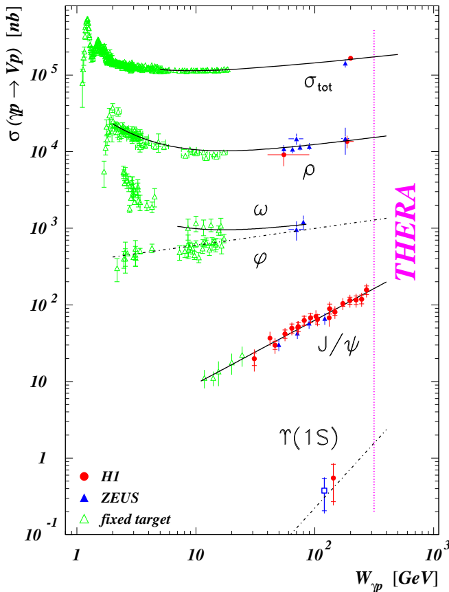
Figure 1.2.4: Energy dependence of the total \gamma p cross section and the elastic vector meson photoproduction cross sections for \rho^0 , \omega , \phi , J/\psi , and \Upsilon mesons. Here W is the photon–proton centre-of-mass energy. The plot is reproduced from [30]. Since the production cross section of heavy vector mesons is proportional to (xg)^2 , measurements in the THERA range of W up to 1 TeV may be sensitive to saturation.
