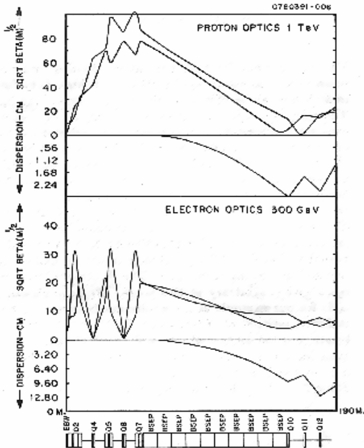
Figure 1.3.1: Possible layout for an electron-proton interaction region, which works for proton/electron energy ratios between one and four. The case for 1 TeV protons and 300 GeV electrons as presented in [126] is shown. One quadrupole triplet and two doublets focus the electron beam strongly. At the beam envelope waists in between these lenses, strong quadrupole magnets are placed which help to focus primarily the protons. After the two beams are properly focused, at 70 m from the IP, a long soft quadrupole magnet, which is aligned along the electron beam orbit, smoothly bends the protons away. This arrangement avoids any extra upstream synchrotron radiation by the beam separation.
