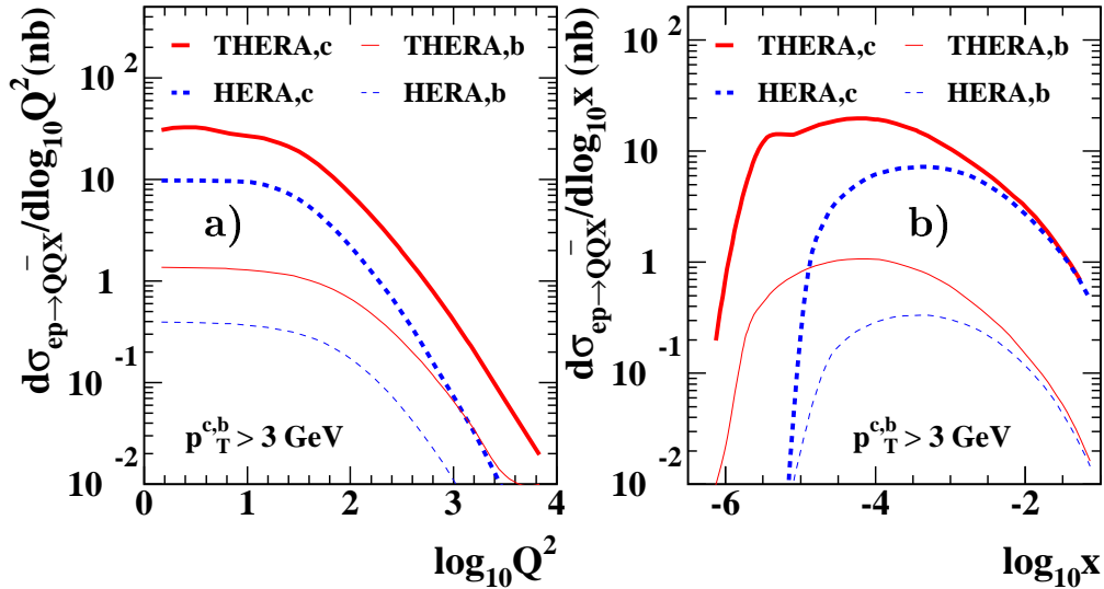
Figure 1.2.13: The differential cross sections for charm (thick curves) and beauty (thin curves) production in neutral current DIS calculated in NLO QCD, (a) d\sigma/d\log_{10} Q^2 and (b) d\sigma/d\log_{10} x . The cross sections at THERA (solid curves) and HERA (dashed curves) are compared.
