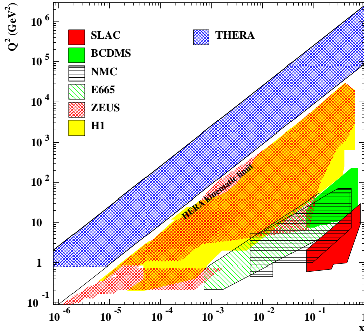
Figure 1.1.1: The kinematic plane in deep inelastic lepton–proton scattering, showing the regions covered by fixed-target scattering experiments and by the HERA experiments, and the extension of the kinematic range by the THERA collider with an ep centre-of-mass energy squared of s = 2.56 \times 10^6 \text{ GeV}^2 . The variables x and Q^2 denote the Bjorken scaling variable and the negative square of the four-momentum transfer between lepton and proton, respectively.
