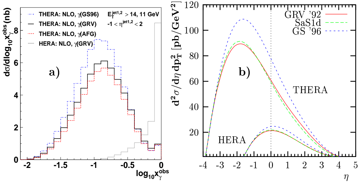
Figure 1.2.20: (a) The differential cross section, d\sigma/d\log_{10} x_\gamma^{\text{obs}} , for inclusive dijet photoproduction at HERA and THERA as predicted by a NLO calculation. (b) The differential cross section for photoproduction of charm in ep reactions, ep \rightarrow e c \bar{c} X , at p_T = 10 \text{ GeV} calculated in LO in the massless (VFNS) scheme.
