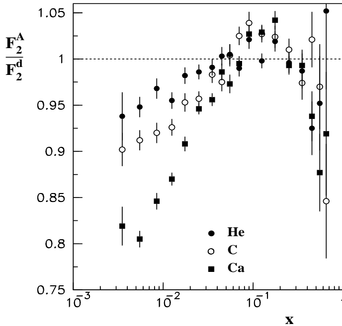
Figure 1.4.1: NMC data [131] for the structure function ratio F_2^A/F_2^d per nucleon for {}^4\text{He} , {}^{12}\text{C} and {}^{40}\text{Ca} for Q^2 \geq 0.7 \text{ GeV}^2 . THERA would extend these measurements by three orders of magnitude to x \simeq 10^{-5} .
