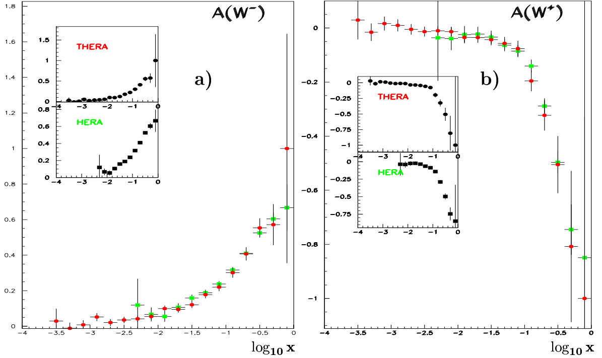
Figure 1.4.5: Simulated measurements of (a) the asymmetry A^{W^-} and (b) of A^{W^+} in CC scattering as functions of x , as expected at the HERA and THERA facilities with polarised proton beams. Note that this representation hides the large differences in the Q^2 range of the HERA and THERA measurements, respectively.
