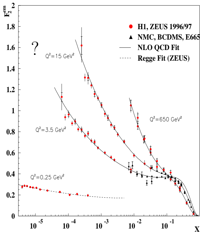
Figure 1.2.1: The proton structure function F_2(x, Q^2) as measured in fixed-target \mu p scattering at large x , and in ep scattering at HERA. The solid curves show a fit using the next-to-leading order QCD evolution equations. The dashed curve for the lowest- Q^2 data is a fit using Regge theory. The structure function in the low- x region represents the sea-quark component of the proton. With THERA, the kinematic range will be extended by a further order of magnitude towards lower x . The expected behaviour of F_2 in this new region is hotly debated.
