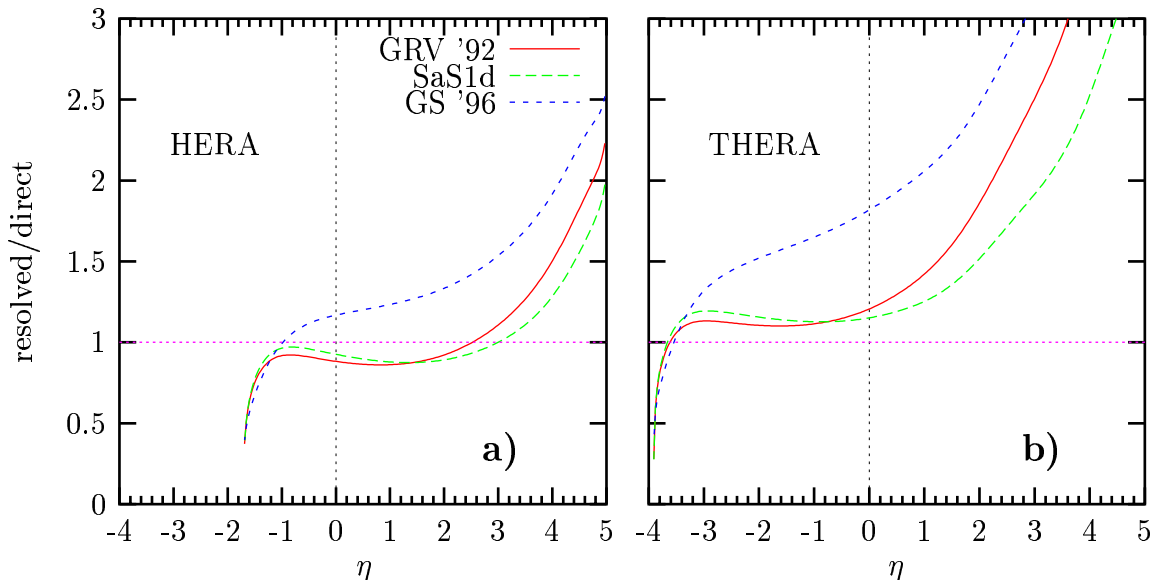
Figure 1.2.21: The ratio of the resolved to the direct contributions to the charm photoproduction cross sections d^2\sigma/d\eta dp_T^2 in ep reactions at p_T = 10 GeV, (a) for HERA and (b) for THERA. The cross sections have been calculated to LO in the massless (VFNS) scheme, using the CTEQ5L parton distribution set for the proton and three different LO parton distribution sets for the photon.
