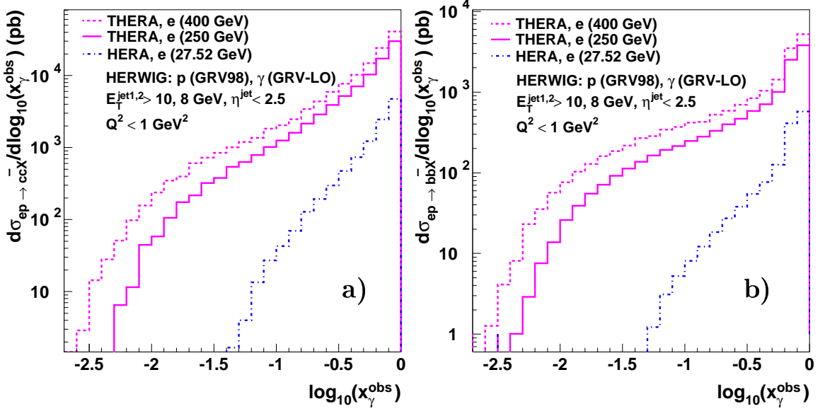
Figure 1.2.12: The differential cross sections d\sigma/d\log_{10} x_{\gamma}^{\text{obs}} for (a) charm and (b) beauty dijet photoproduction as calculated in LO with the Monte Carlo generator HERWIG. The cross sections are shown for THERA, for a proton beam energy of 920 GeV and electrons with 250 GeV (solid magenta) and 400 GeV (dashed magenta), and for HERA (dashed blue).
