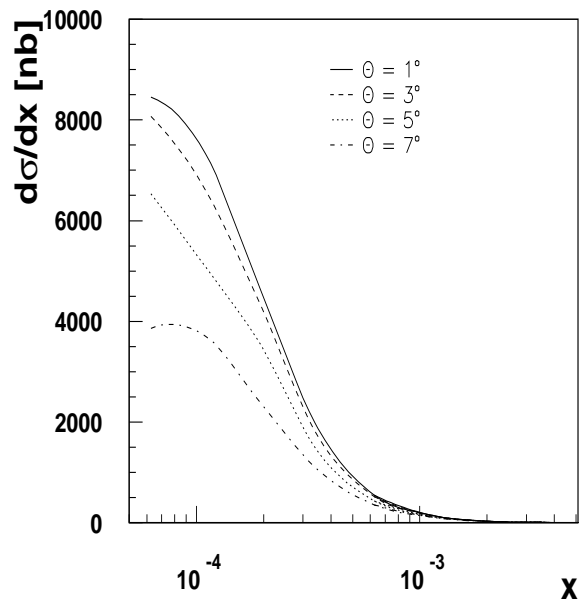
Figure 1.2.10: Forward-jet cross section as a function of x obtained from CCFM for 0.5 < p_t^2/Q^2 < 2 , for different values of the minimum jet angle.
