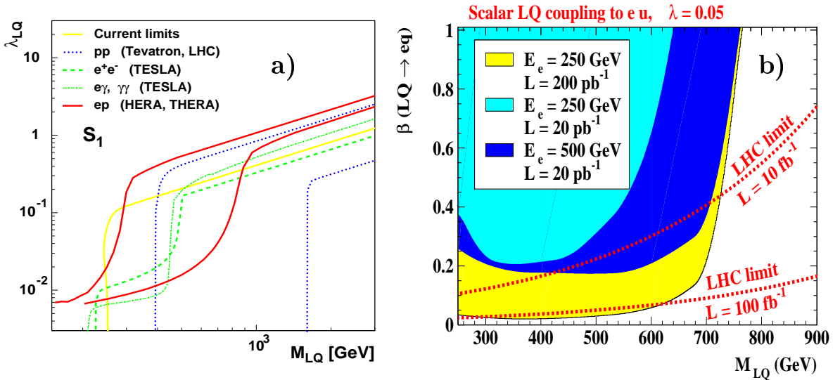
Figure 1.2.17: (a) Mass-dependent upper bounds on the LQ coupling \lambda as expected at THERA (lower solid red curve, E_e = 250 \text{ GeV} , E_p = 920 \text{ GeV} , 100 \text{ pb}^{-1} of e^-p data), HERA (upper solid red curve, 2 \times 400 \text{ pb}^{-1} of e^\pm p data), TESLA ( E_e = 250 \text{ GeV} , 100 \text{ fb}^{-1} of ee , e\gamma or \gamma\gamma data), Tevatron (upper dotted curve, 10 \text{ fb}^{-1} ) and LHC (lower dotted curve, \sqrt{s} = 14 \text{ TeV} , 100 \text{ fb}^{-1} ). Upper limits as obtained from a global fit of various existing data sets [104] are also shown by the solid yellow curve. (b) Typical expected mass-dependent sensitivities on the branching ratio \beta(LQ \rightarrow eq) of a LQ decaying to eq , at THERA for two different values of the lepton beam energy and at LHC; the coloured regions (the domains above the dashed red curves) would be probed by THERA (LHC).
