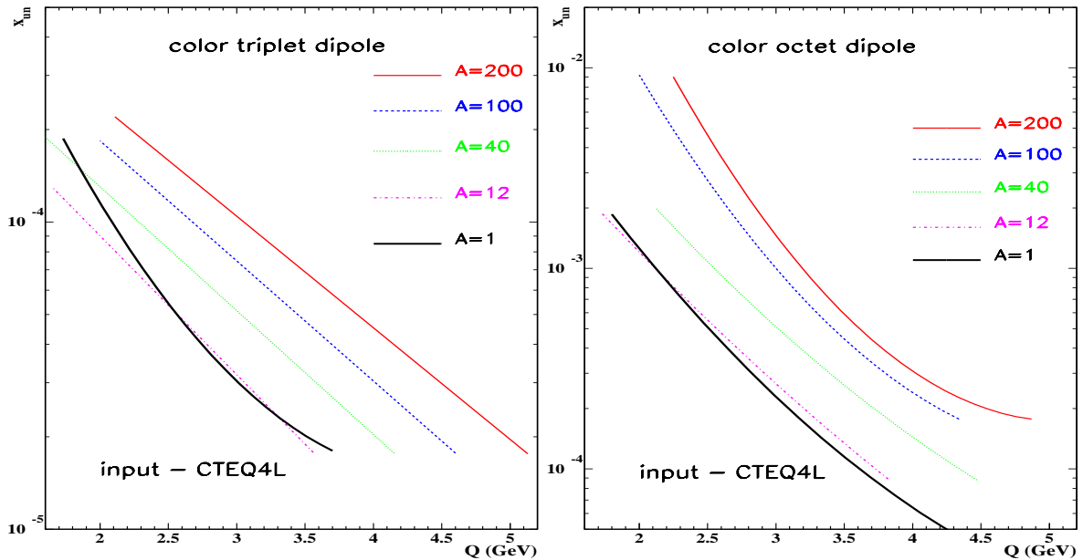
Figure 1.4.2: Unitarity boundaries in the (x, \sqrt{Q^2}) -plane for (a) the inelastic q\bar{q} (colour triplet)–nucleus and (b) the q\bar{q}g (colour octet)–nucleus cross sections for nuclei with A = 12, 40, 100 and 200 . The unitarity boundaries for the inelastic q\bar{q} – and q\bar{q}g –nucleon cross sections are indicated as black solid lines.
