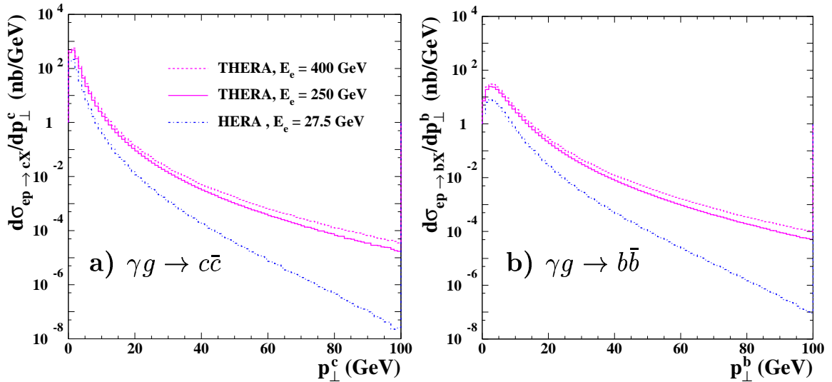
Figure 1.2.11: The contribution of photon–gluon fusion to the differential cross sections d\sigma/dp_{\perp} for (a) charm and (b) beauty production calculated in NLO QCD for Q^2 < 1 \text{ GeV}^2 . The solid and dashed violet curves show the predictions for THERA operation with an electron energy of 250 \text{ GeV} and 400 \text{ GeV} , respectively, and E_p = 920 \text{ GeV} . The predictions for the HERA case are indicated by the dash-dotted blue curves.
