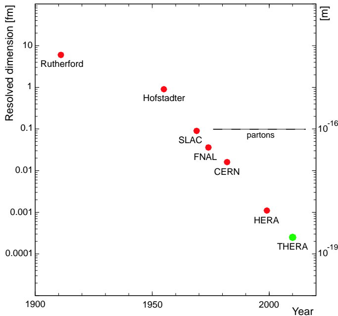
Figure 1.1.2: The development over time of the resolution power of experiments exploring the inner structure of matter, from the Rutherford experiment to THERA.
