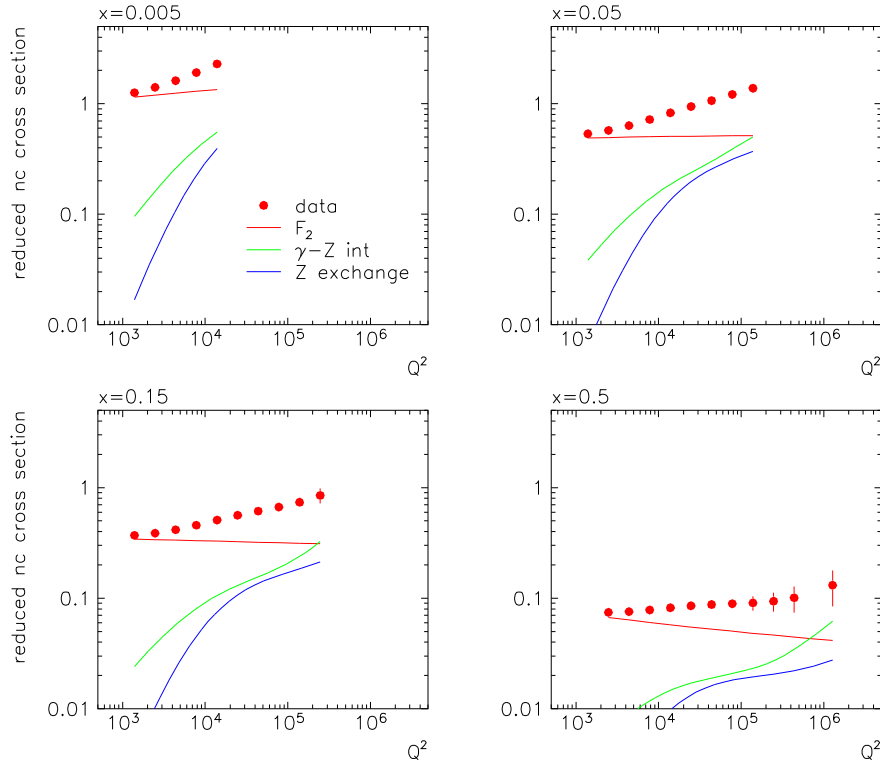
Figure 1.2.15: Simulation of a measurement of the reduced NC DIS cross section at THERA in unpolarised electron scattering, for an integrated luminosity of 200 \text{ pb}^{-1} . The error bars are a convolution of statistical and estimated systematic uncertainties. The curves represent the fraction of the one-photon exchange (red, top), of the \gamma Z interference (green, middle) and of the pure Z exchange (blue, bottom). Towards very high Q^2 , depending on the lepton beam charge and polarisation, the Z exchange contributions become increasingly important.
