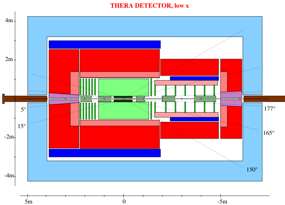
Figure 1.3.4: Basic design of the THERA detector in the low- x configuration. The electrons enter from left, the protons from right. Around the beam-pipe, modules of 6-inch silicon strip detectors are positioned (dark-green). Tracking is complemented by planar and circular track chambers (light-green). Electromagnetic (pink) and hadronic (red) calorimetry ensures hermetic, accurate reconstruction of the final-state energy depositions. A homogenous, solenoidal field over 9 m length is provided by the large-diameter H1 coil and the smaller ZEUS coil (blue). The return yoke iron structure (light-blue) is instrumented for shower tail catching and muon detection. The focusing magnets (brown) are placed near the plug calorimeters (magenta).
