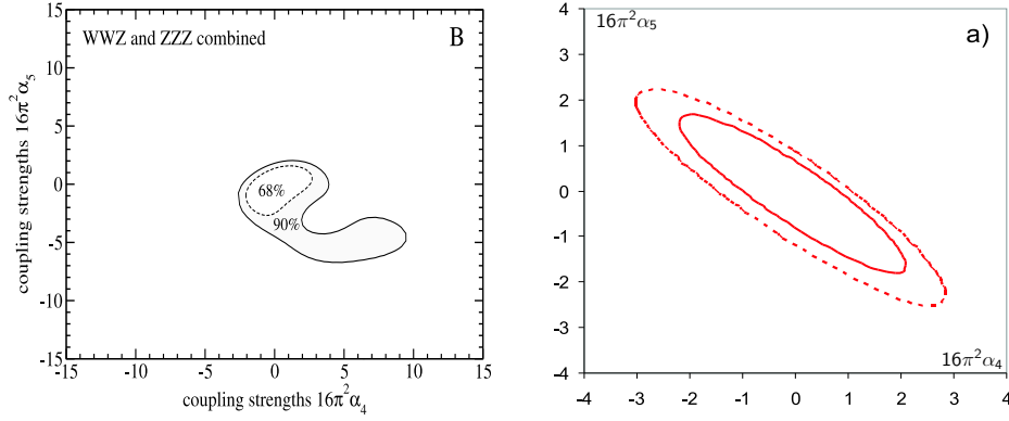
Figure 1: Left: Combined fit for WWZ/ZZZ production at \sqrt{s} = 1 TeV, 1 \text{ ab}^{-1} , both beams polarized. Right: Expected sensitivity (combined fit for all processes) to quartic anomalous couplings for a 1 \text{ ab}^{-1} e^+e^- sample in the conserved SU(2)_c case. Solid lines represent 90% CL, dashed ones 68%.
